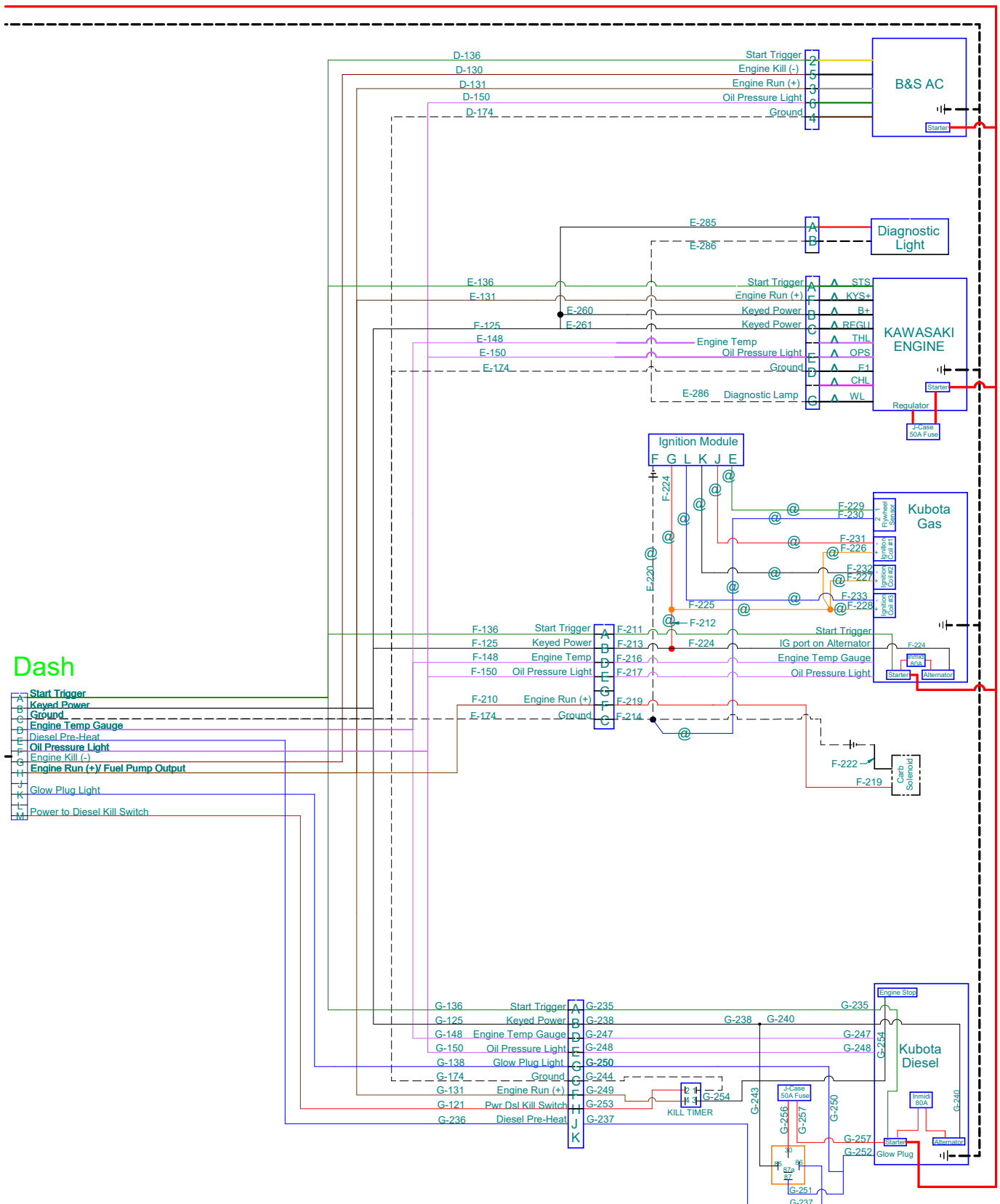
Wiring Diagram - Engine Harness, 1 PTO Fuse Relay (Serial # 01001-02172)
