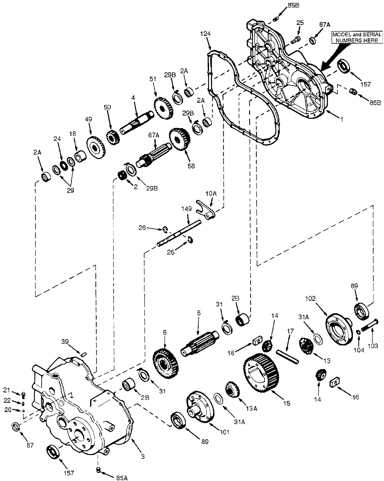
ILLUSTRATED DRAWING Peerless Transaxle (51.0087)
