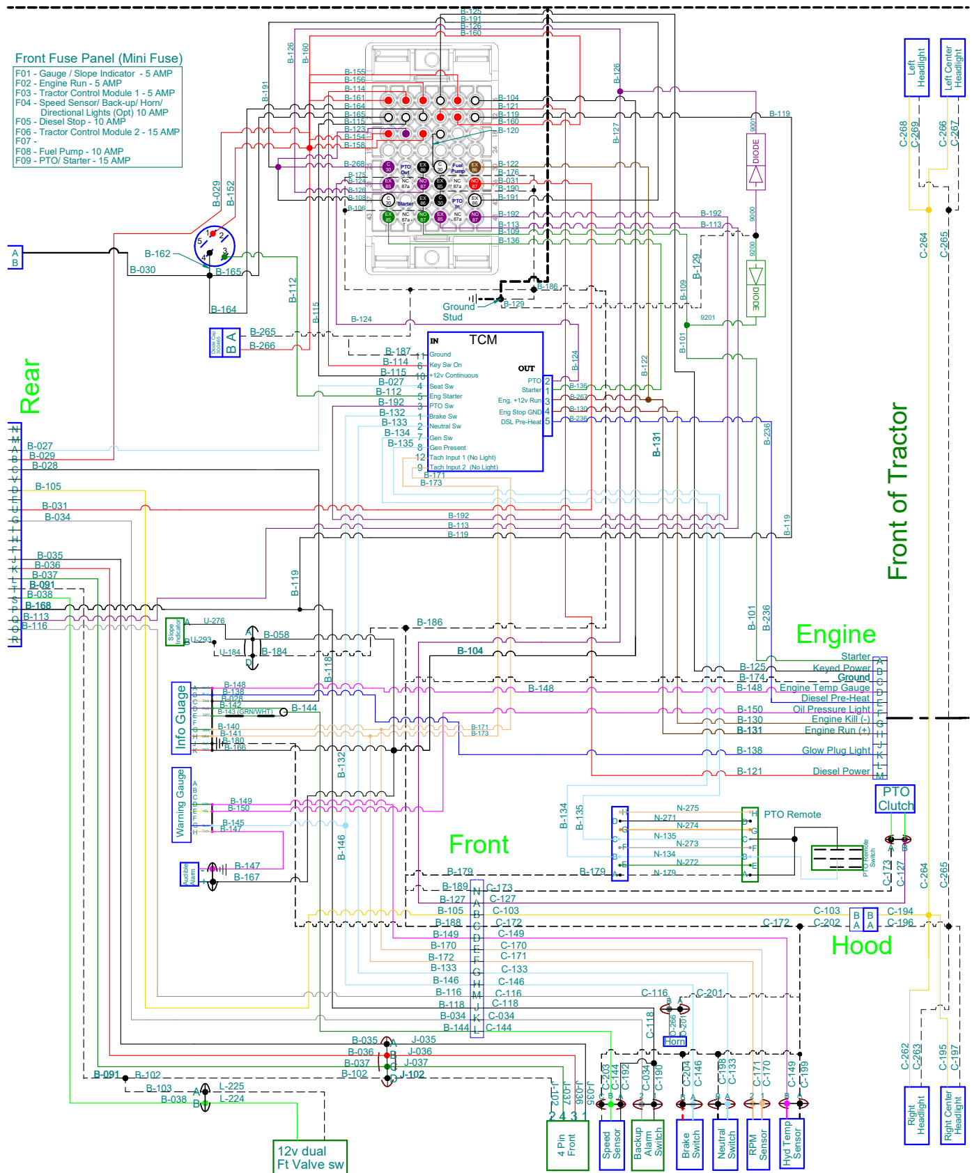
Wiring Diagram - Front Harness (Serial # 02173-05664)
