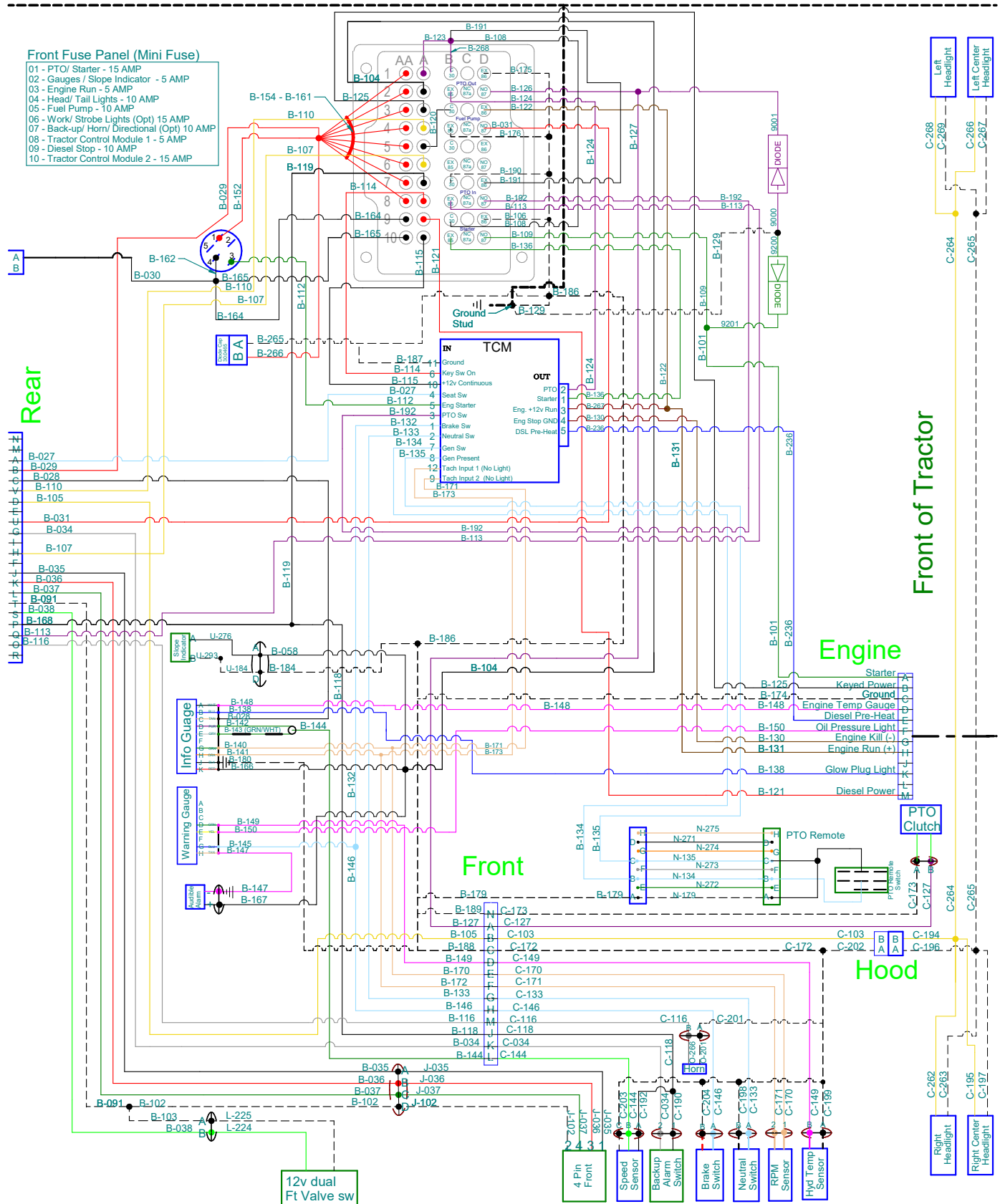
Wiring Diagram - Front Harness, 2 PTO Fuse Relay (Serial # 01001-02172)
