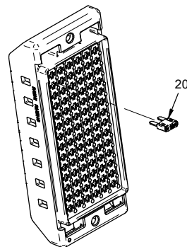
Rear Fuse Panel (Serial # 02233-)
