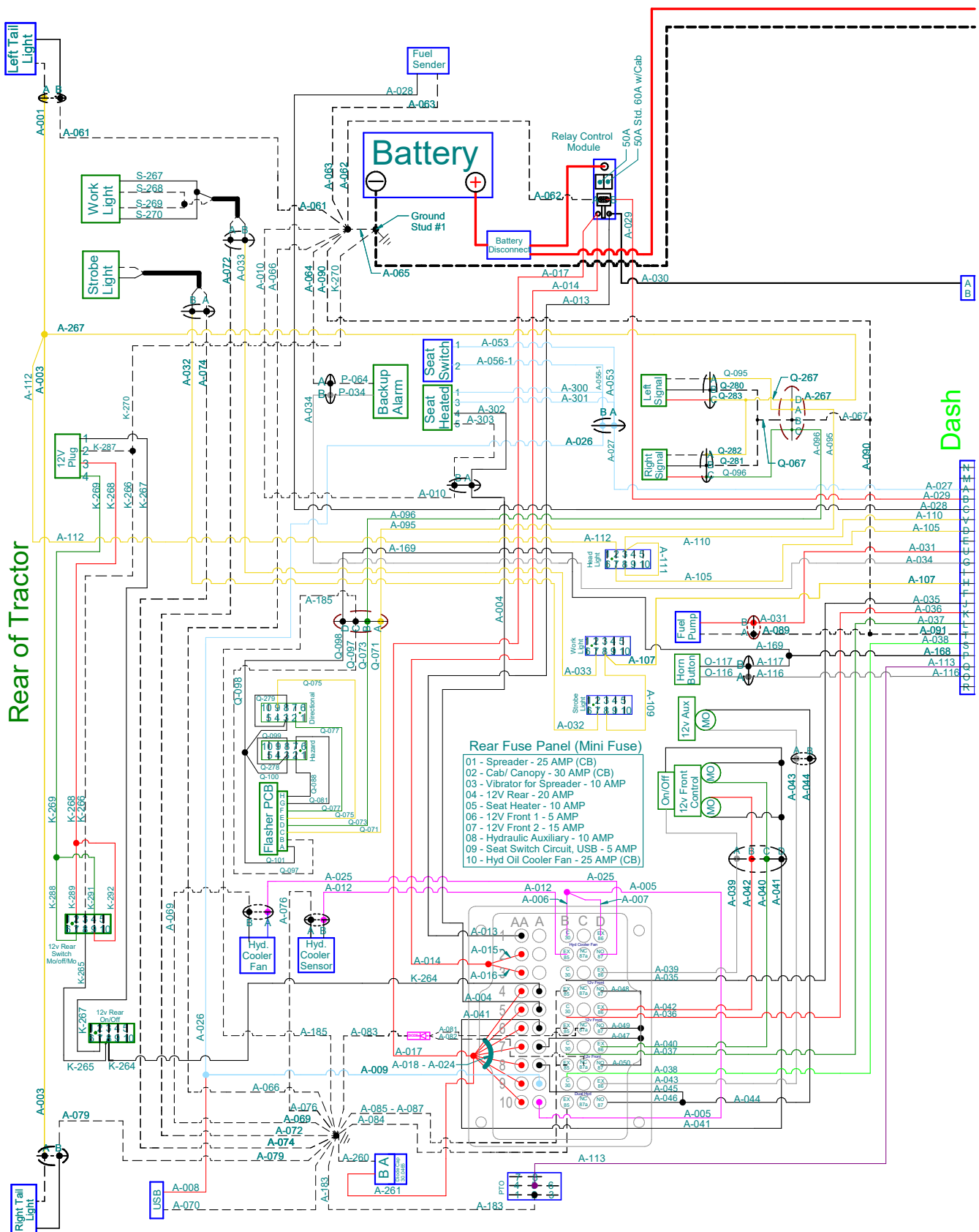
Wiring Diagram - Rear Harness (Serial # 01001-02172)
